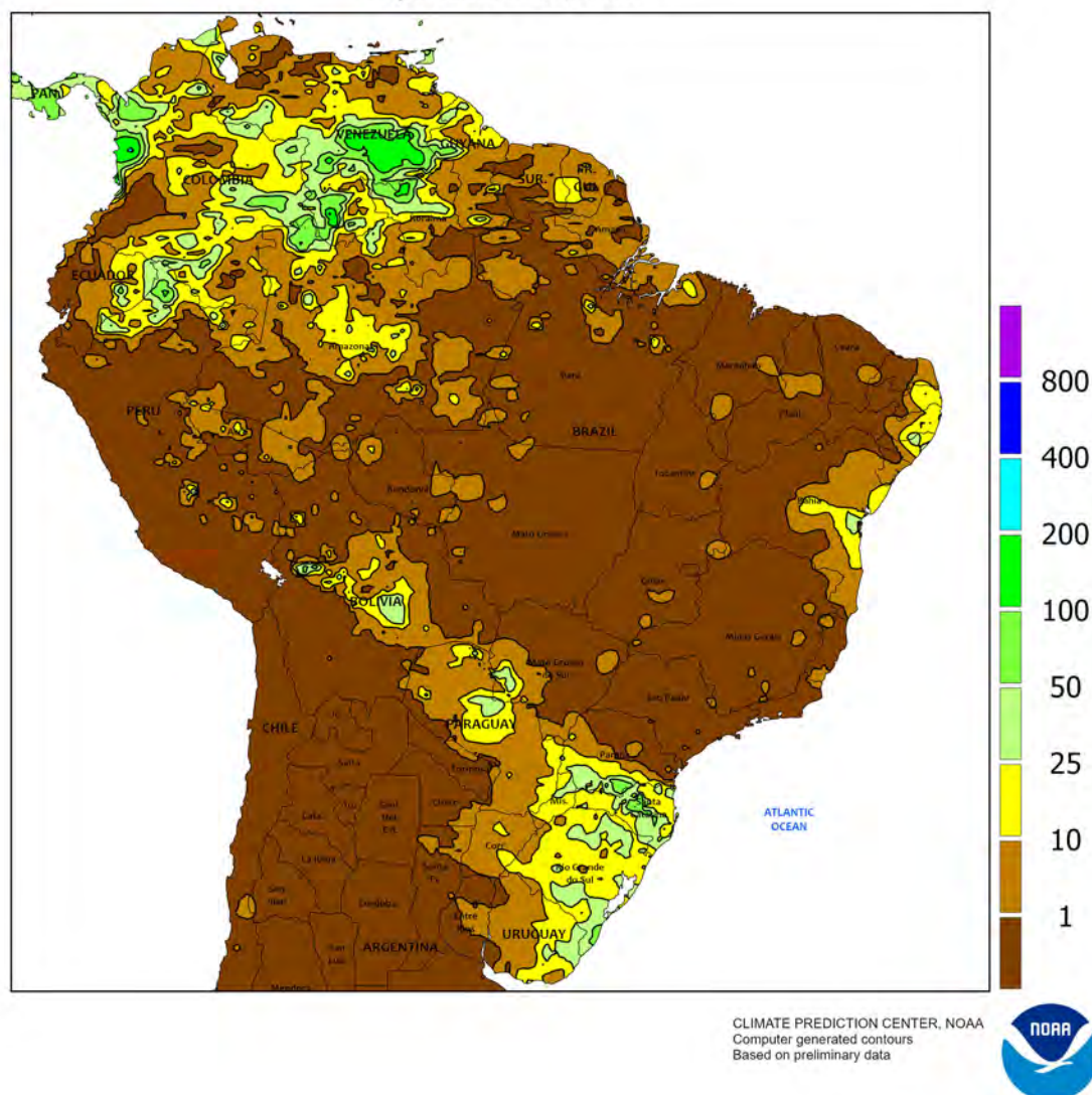
BRAZIL Total Precipitation(mm) September 8 - 14, 2024
