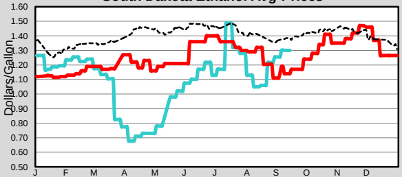
South Dakota Ethanol Avg Prices
